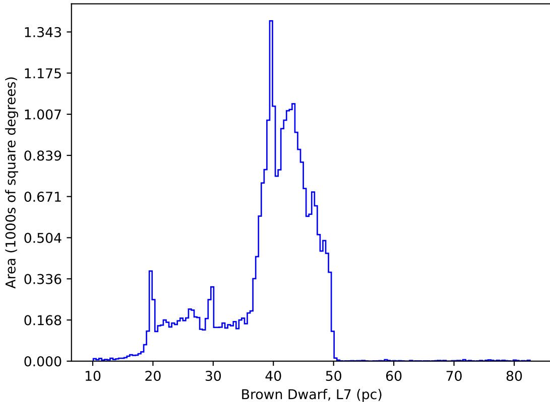
too_ignore_10_1v3.4_10yrs : Brown Dwarf, L7
