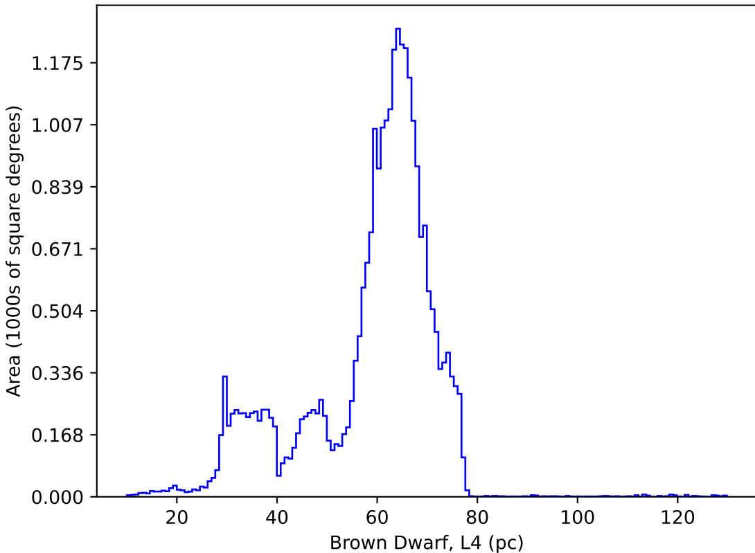
too_ignore_10_1v3.4_10yrs : Brown Dwarf, L4
