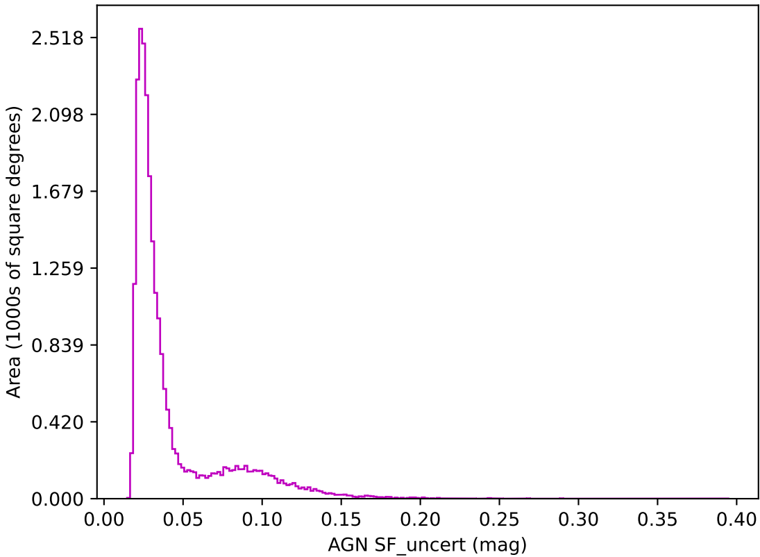
too_ignore_10_1v3.4_10yrs z band: AGN SF_uncert
