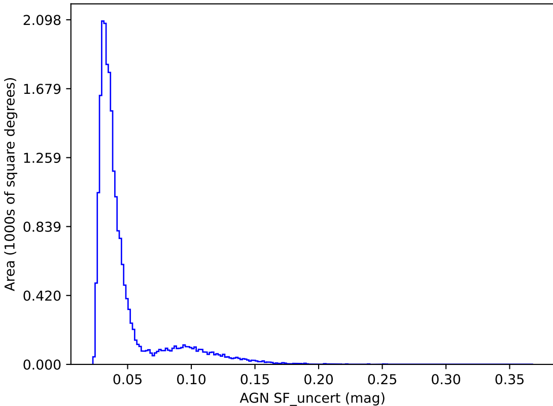
too_ignore_10_1v3.4_10yrs y band: AGN SF_uncert
