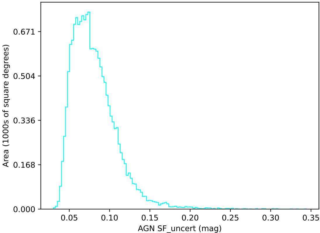
too_ignore_10_1v3.4_10yrs u band: AGN SF_uncert
