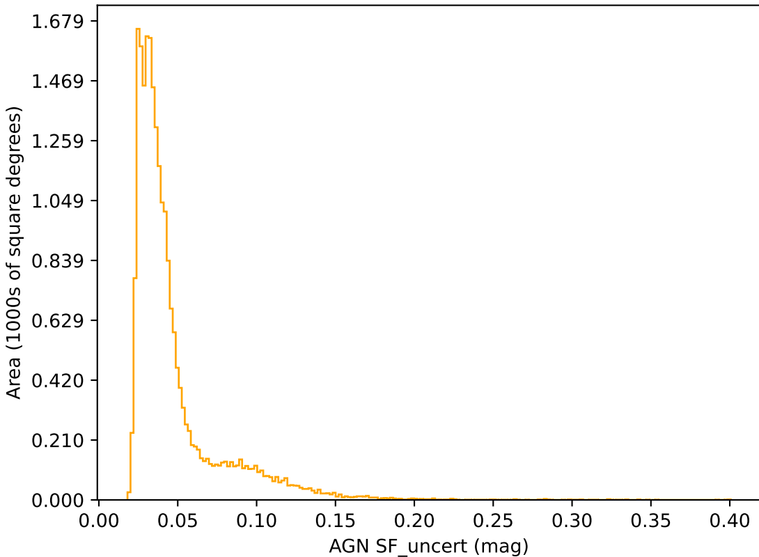
too_ignore_10_1v3.4_10yrs r band: AGN SF_uncert
