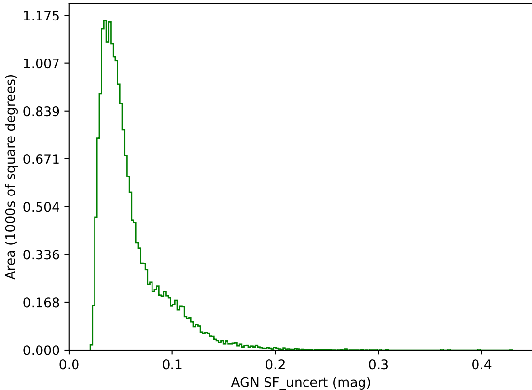
too_ignore_10_1v3.4_10yrs g band: AGN SF_uncert
