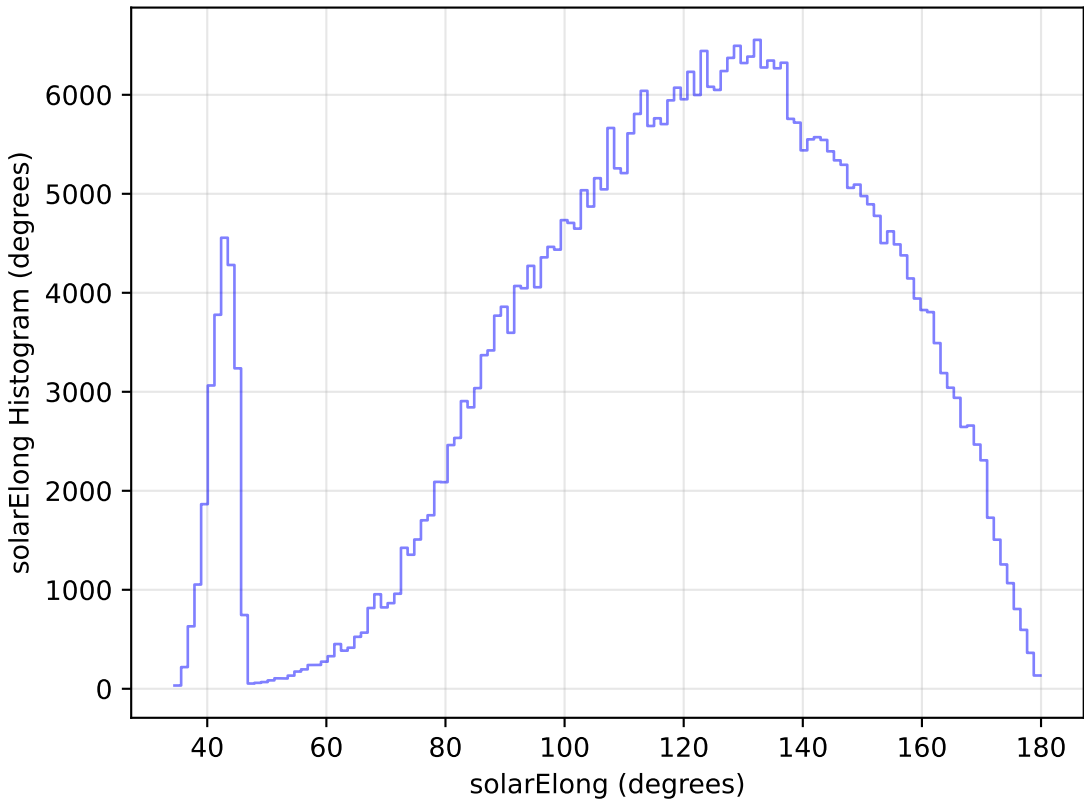
too_ignore_10_1v3.4_10yrs WFD z band: solarElong Histogram
