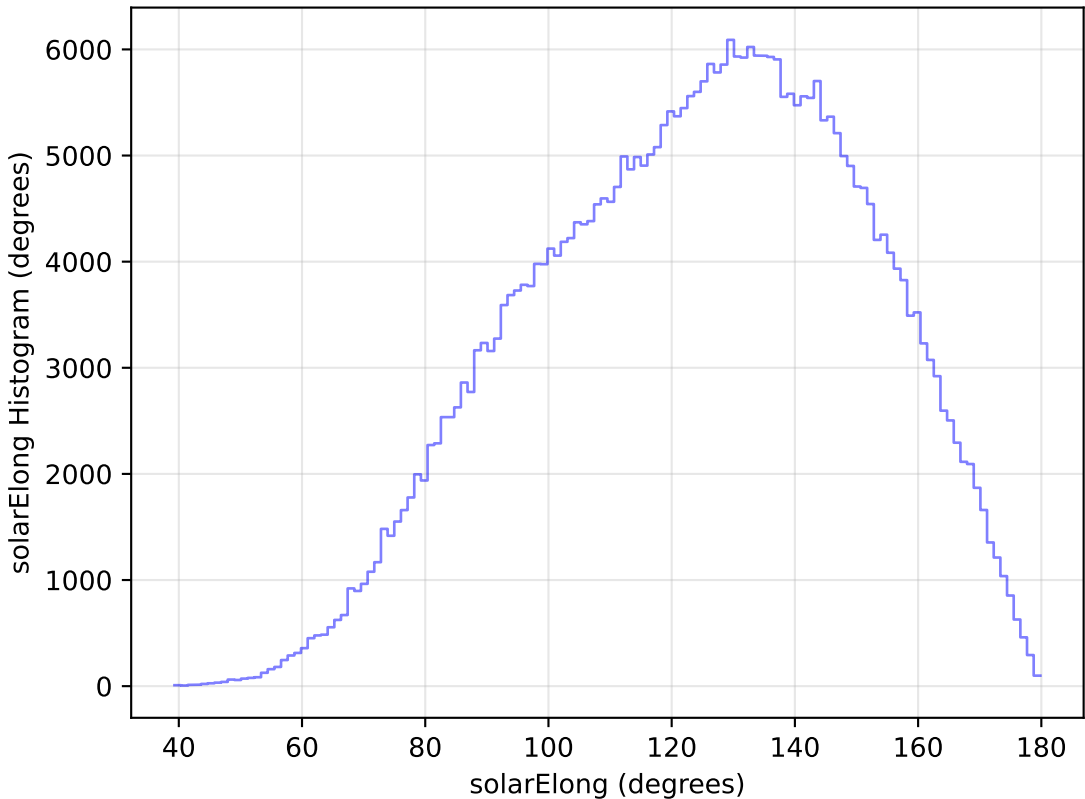
too_ignore_10_1v3.4_10yrs WFD y band: solarElong Histogram
