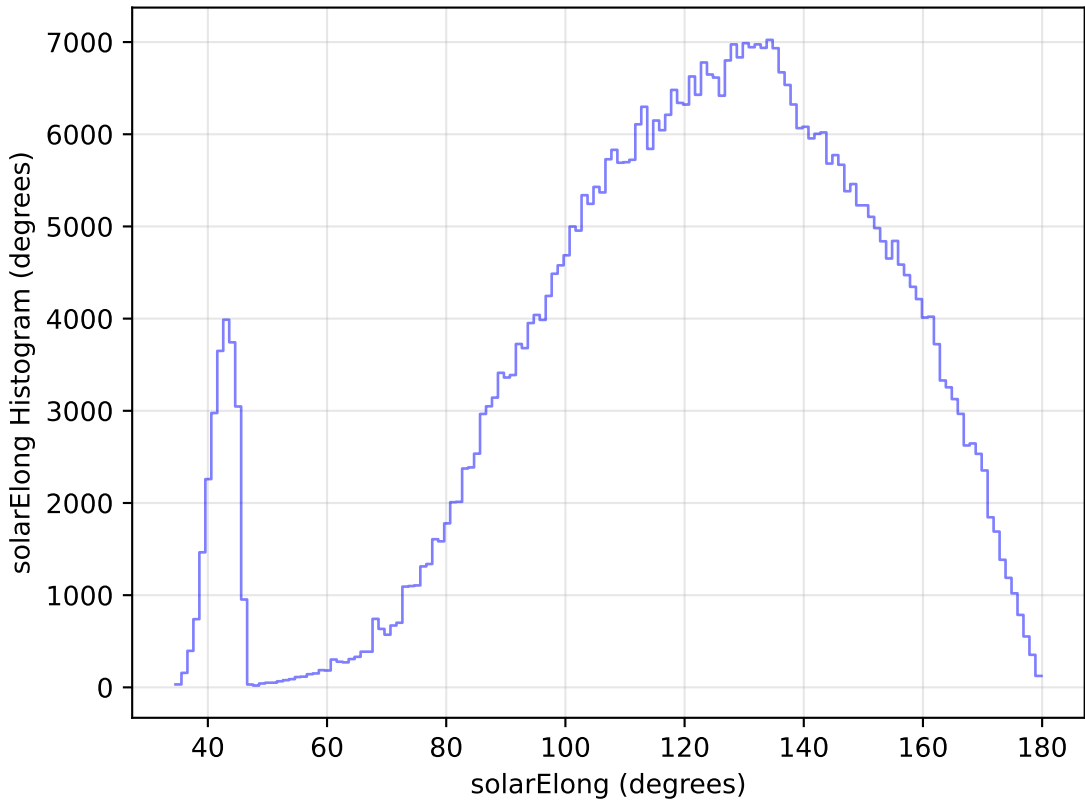
too_ignore_10_1v3.4_10yrs WFD i band: solarElong Histogram
