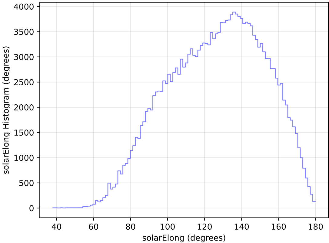
too_ignore_10_1v3.4_10yrs WFD g band: solarElong Histogram
