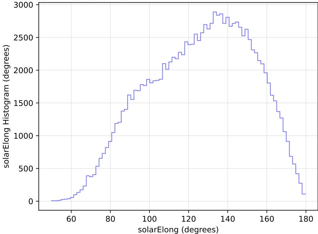
too_ignore_10_1v3.4_10yrs All sky u band: solarElong Histogram
