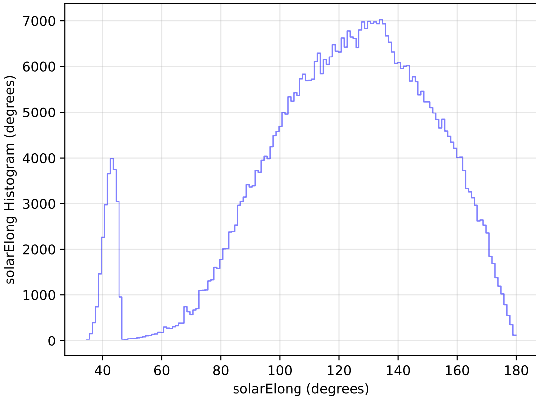
too_ignore_10_1v3.4_10yrs All sky i band: solarElong Histogram
