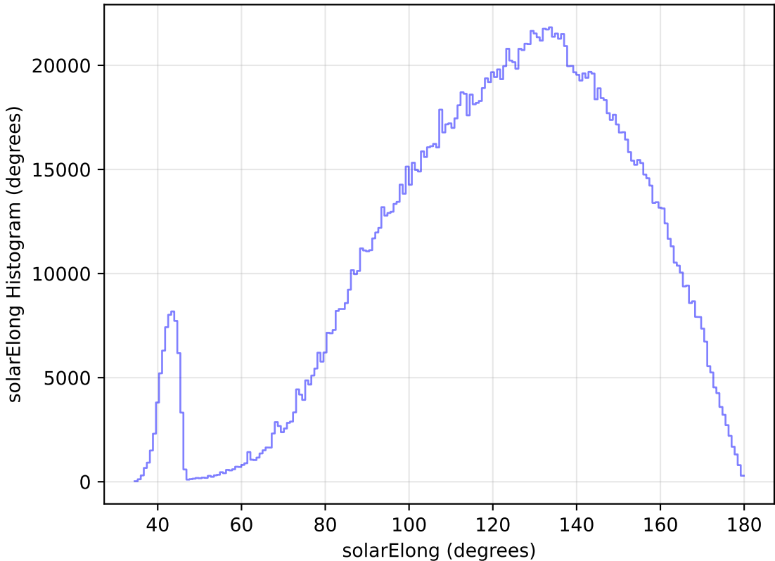
too_ignore_10_1v3.4_10yrs All sky all bands: solarElong Histogram
