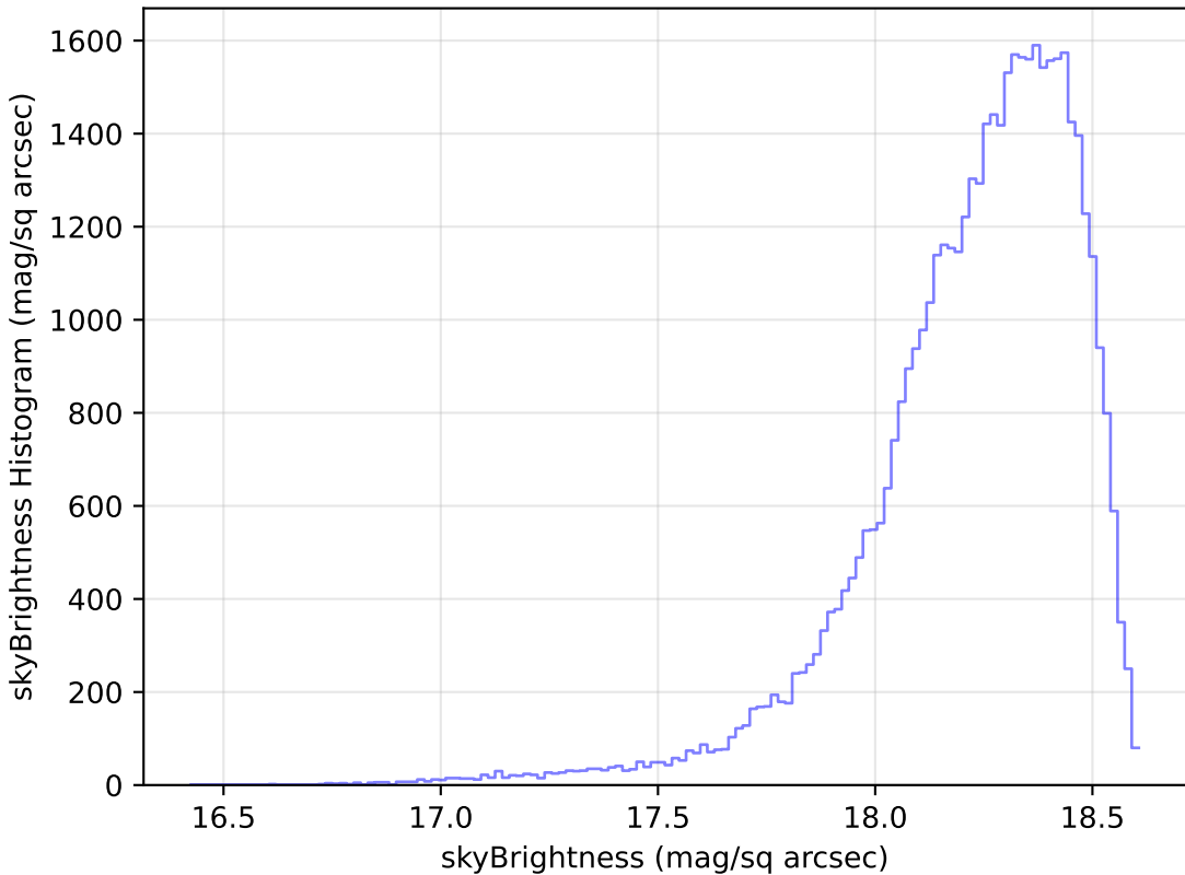
too_ignore_10_1v3.4_10yrs Yr 1 y band: skyBrightness Histogram
