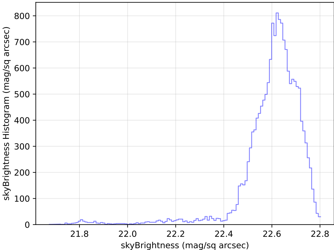
too_ignore_10_1v3.4_10yrs Yr 1 u band: skyBrightness Histogram
