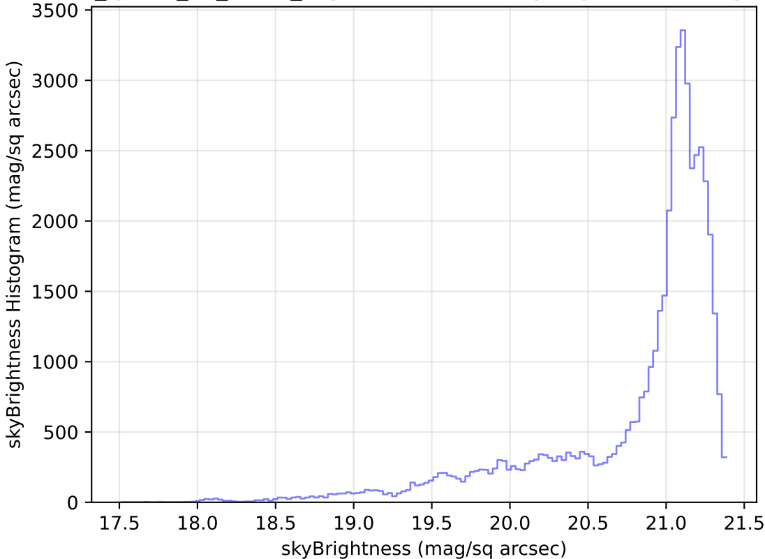
too_ignore_10_1v3.4_10yrs Yr 1 r band: skyBrightness Histogram
