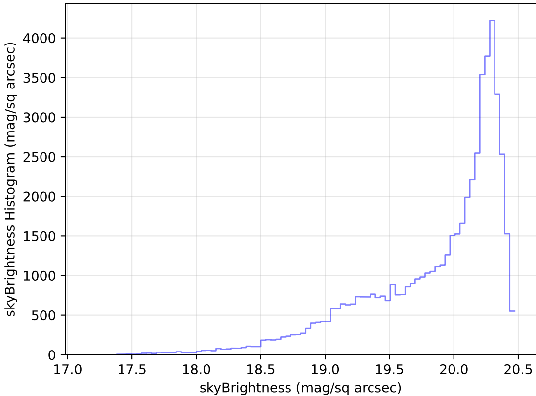
too_ignore_10_1v3.4_10yrs Yr 1 i band: skyBrightness Histogram
