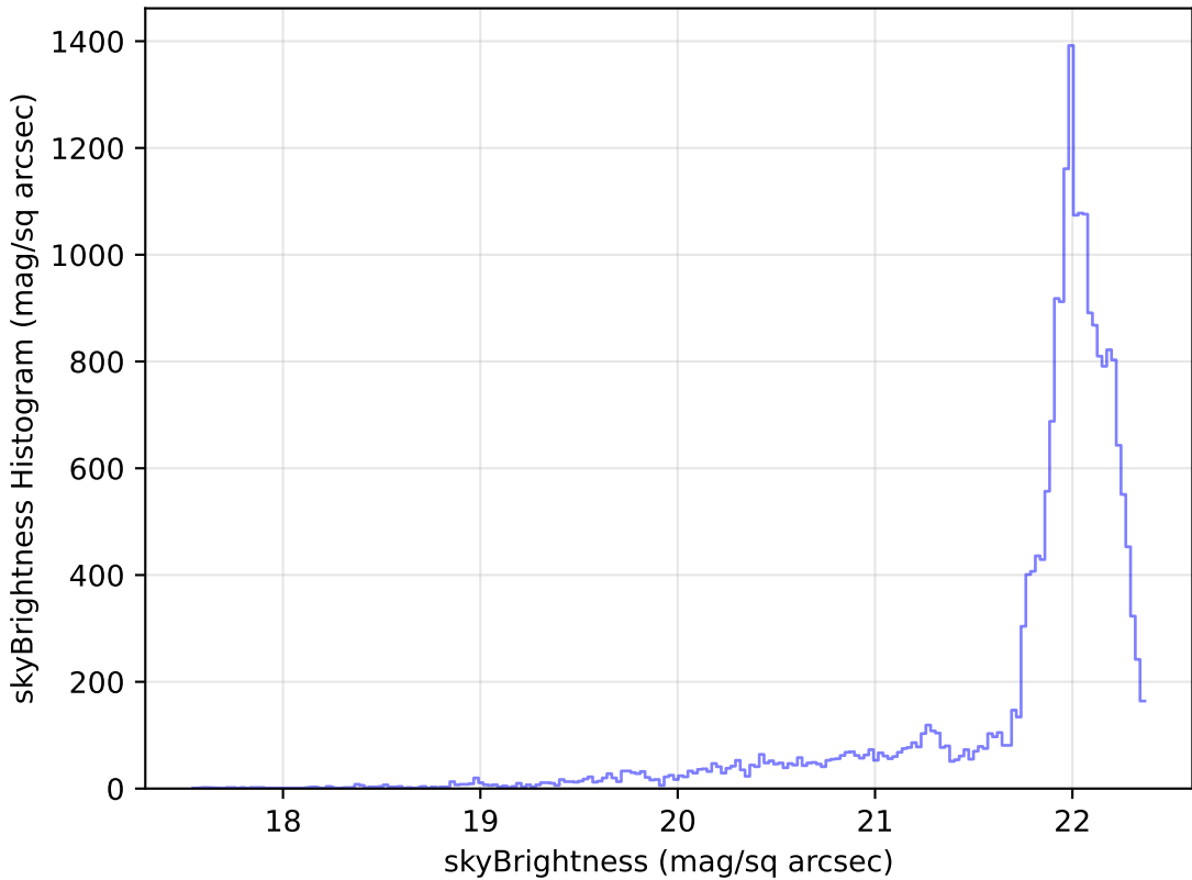
too_ignore_10_1v3.4_10yrs Yr 1 g band: skyBrightness Histogram
