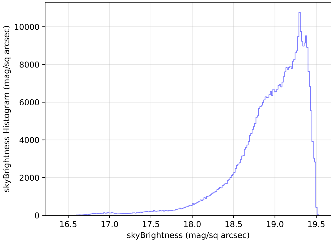
too_ignore_10_1v3.4_10yrs WFD z band: skyBrightness Histogram
