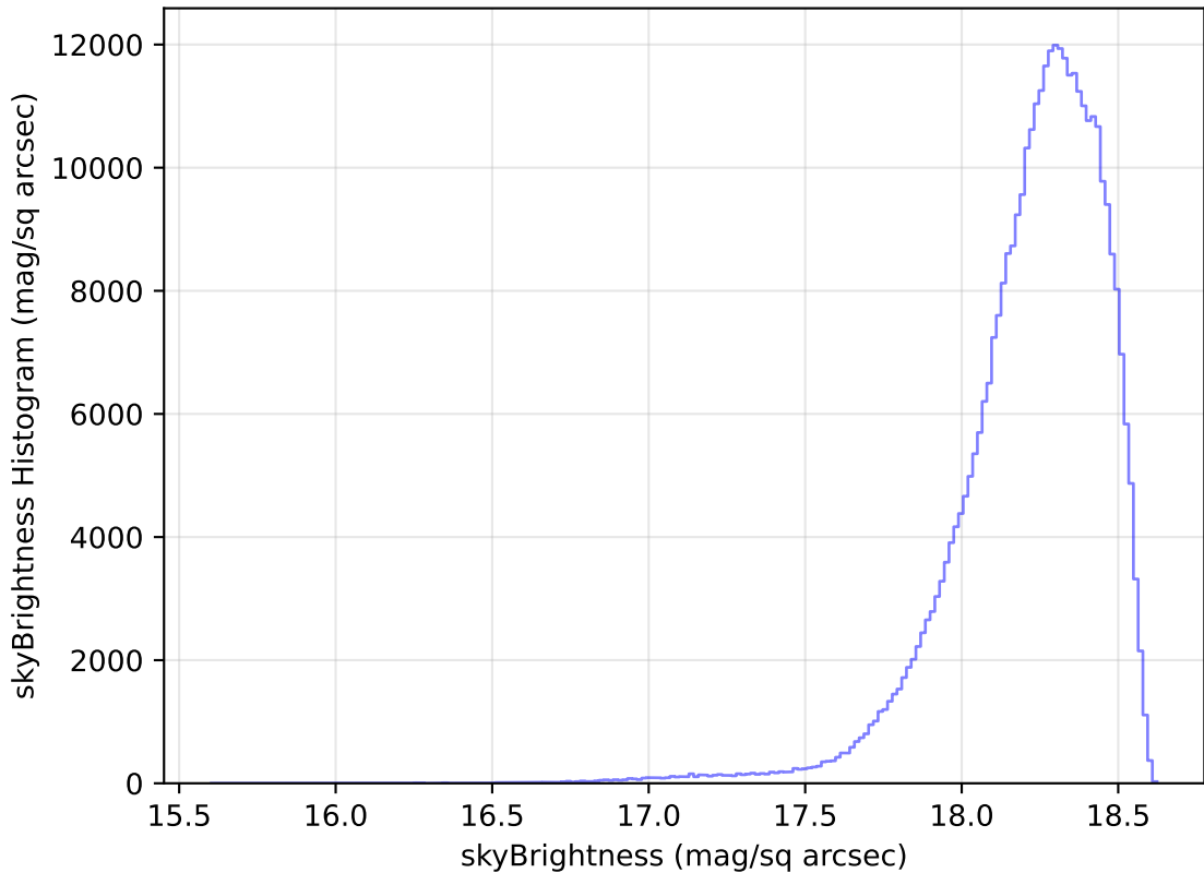
too_ignore_10_1v3.4_10yrs WFD y band: skyBrightness Histogram
