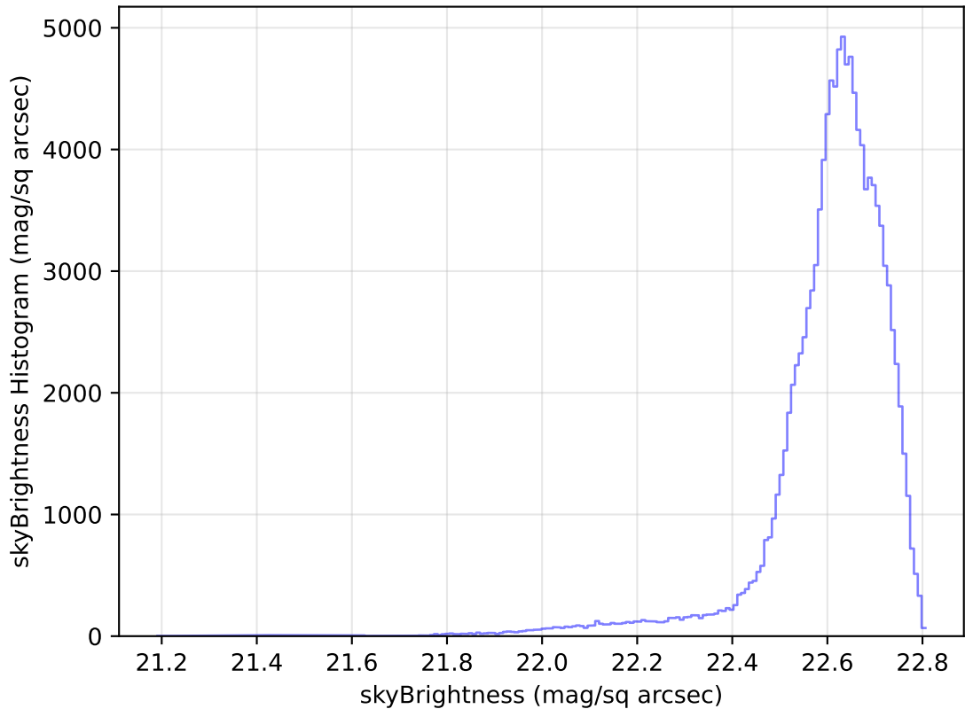
too_ignore_10_1v3.4_10yrs WFD u band: skyBrightness Histogram
