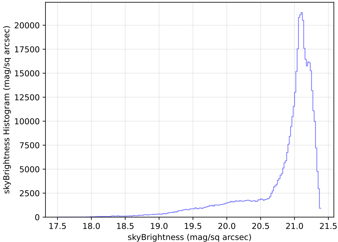
too_ignore_10_1v3.4_10yrs WFD r band: skyBrightness Histogram
