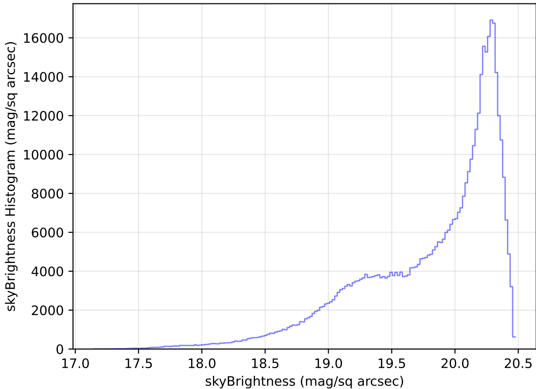
too_ignore_10_1v3.4_10yrs WFD i band: skyBrightness Histogram
