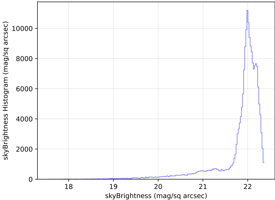
too_ignore_10_1v3.4_10yrs WFD g band: skyBrightness Histogram
