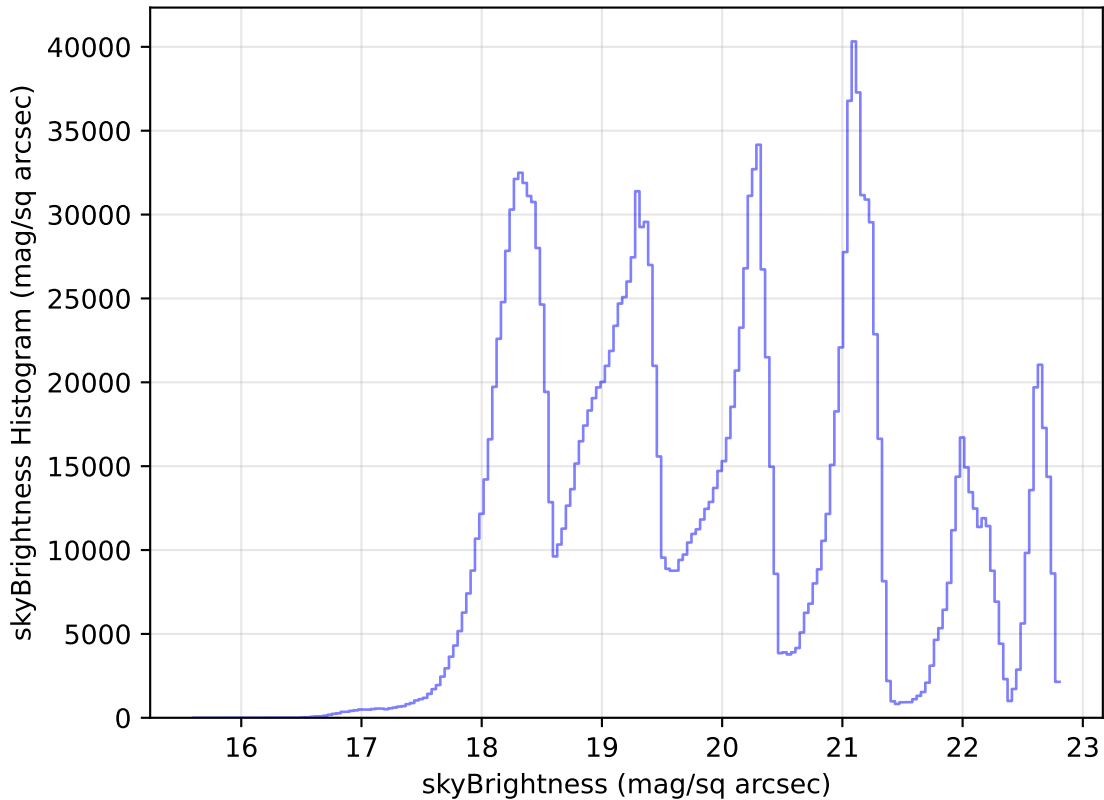
too_ignore_10_1v3.4_10yrs WFD all bands: skyBrightness Histogram
