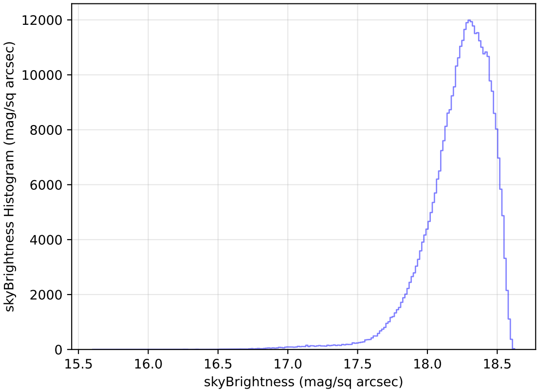
too_ignore_10_1v3.4_10yrs All sky y band: skyBrightness Histogram
