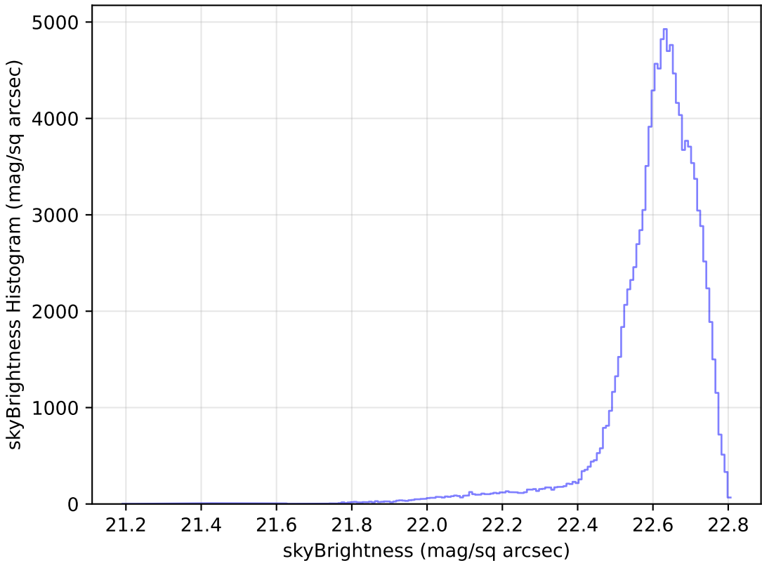
too_ignore_10_1v3.4_10yrs All sky u band: skyBrightness Histogram
