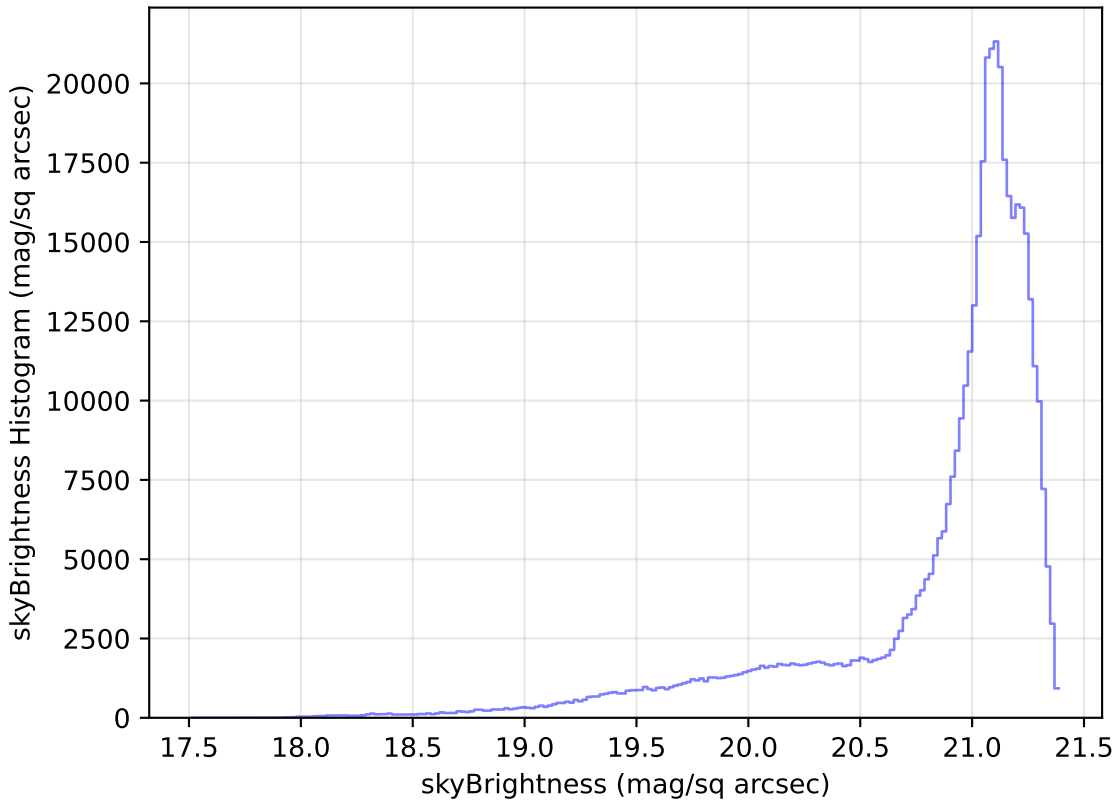
too_ignore_10_1v3.4_10yrs All sky r band: skyBrightness Histogram
