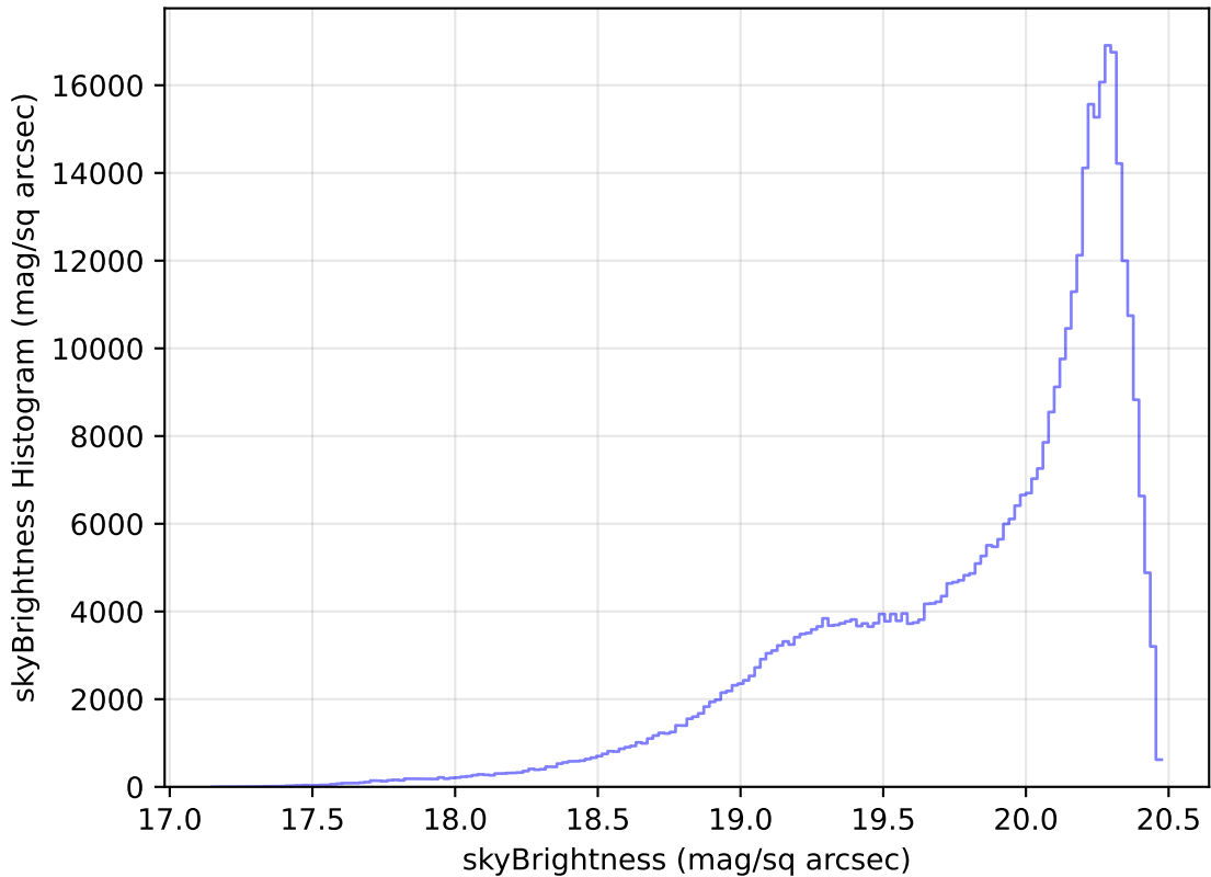
too_ignore_10_1v3.4_10yrs All sky i band: skyBrightness Histogram
