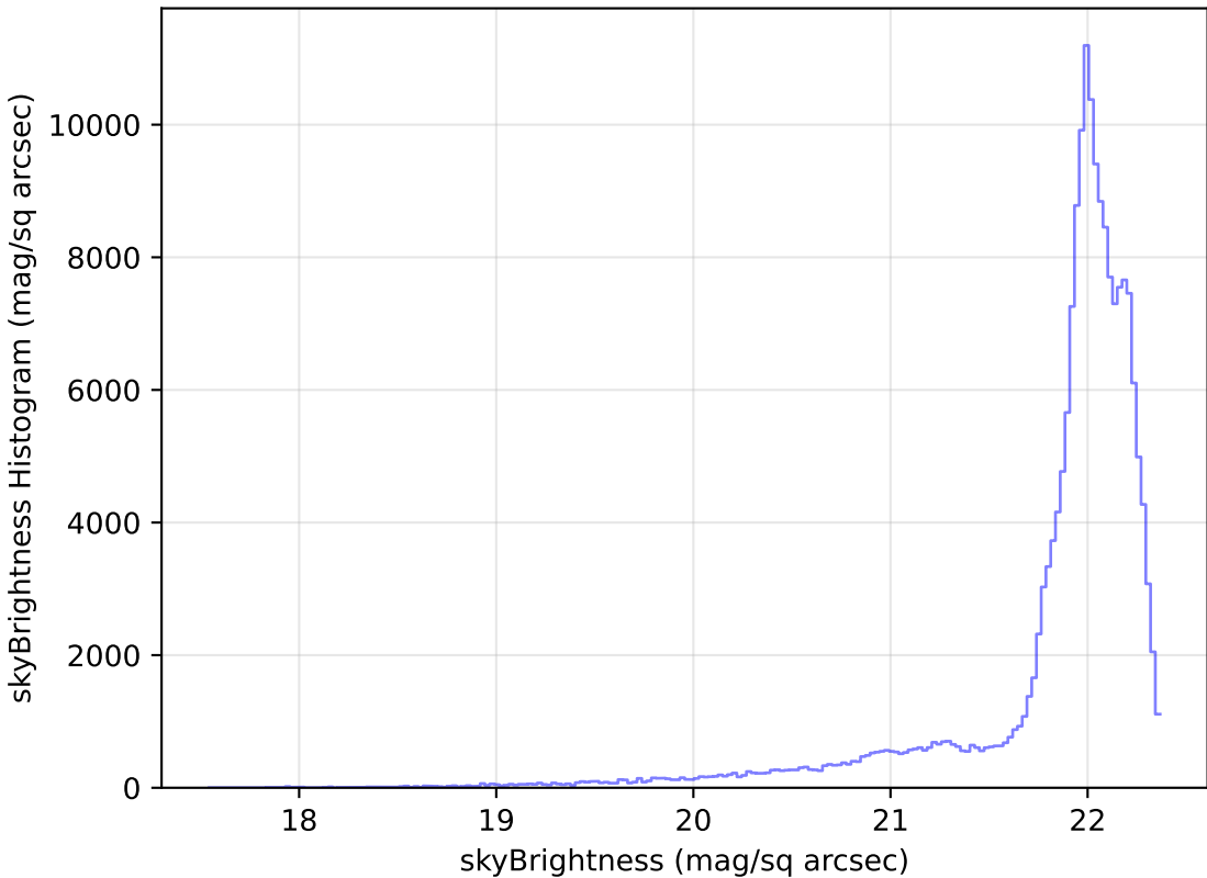
too_ignore_10_1v3.4_10yrs All sky g band: skyBrightness Histogram
