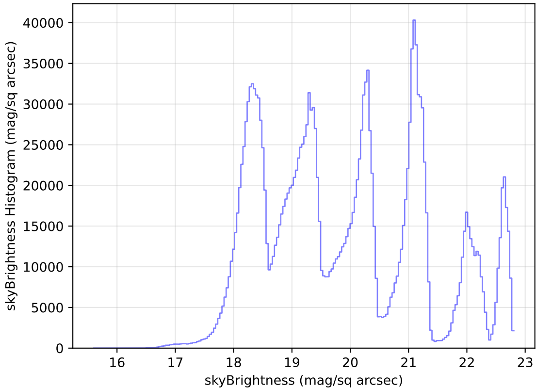
too_ignore_10_1v3.4_10yrs All sky all bands: skyBrightness Histogram
