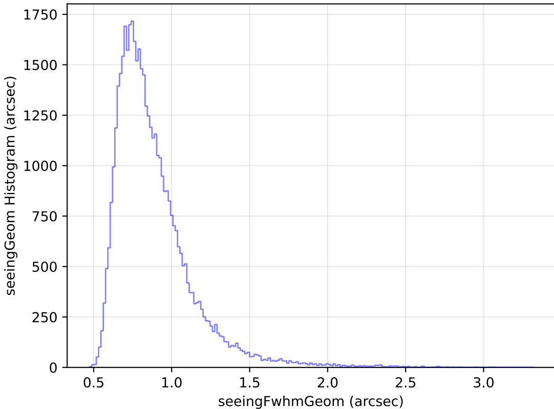
too_ignore_10_1v3.4_10yrs Yr 1 z band: seeingGeom Histogram
