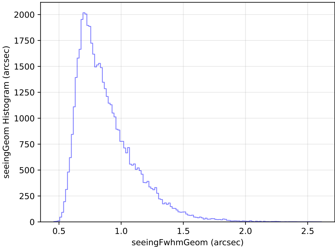
too_ignore_10_1v3.4_10yrs Yr 1 r band: seeingGeom Histogram
