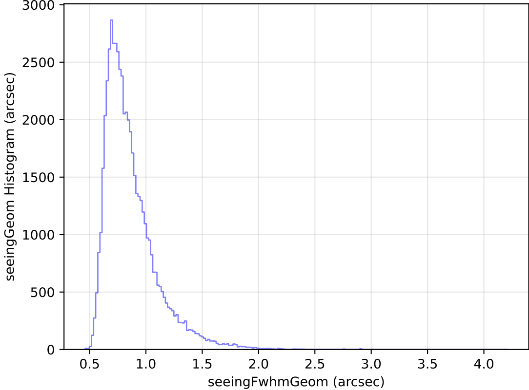
too_ignore_10_1v3.4_10yrs Yr 1 i band: seeingGeom Histogram
