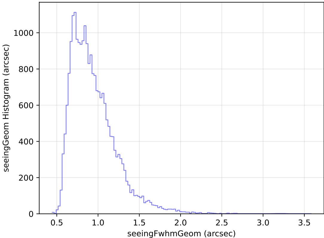
too_ignore_10_1v3.4_10yrs Yr 1 g band: seeingGeom Histogram
