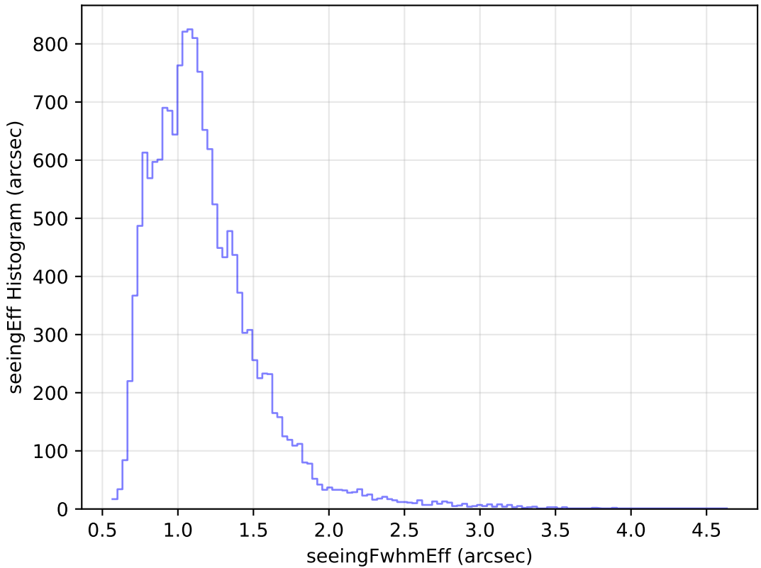
too_ignore_10_1v3.4_10yrs Yr 1 u band: seeingEff Histogram
