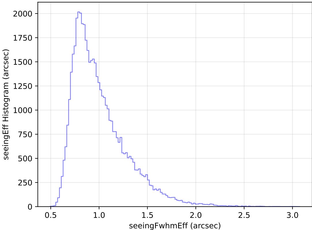
too_ignore_10_1v3.4_10yrs Yr 1 r band: seeingEff Histogram
