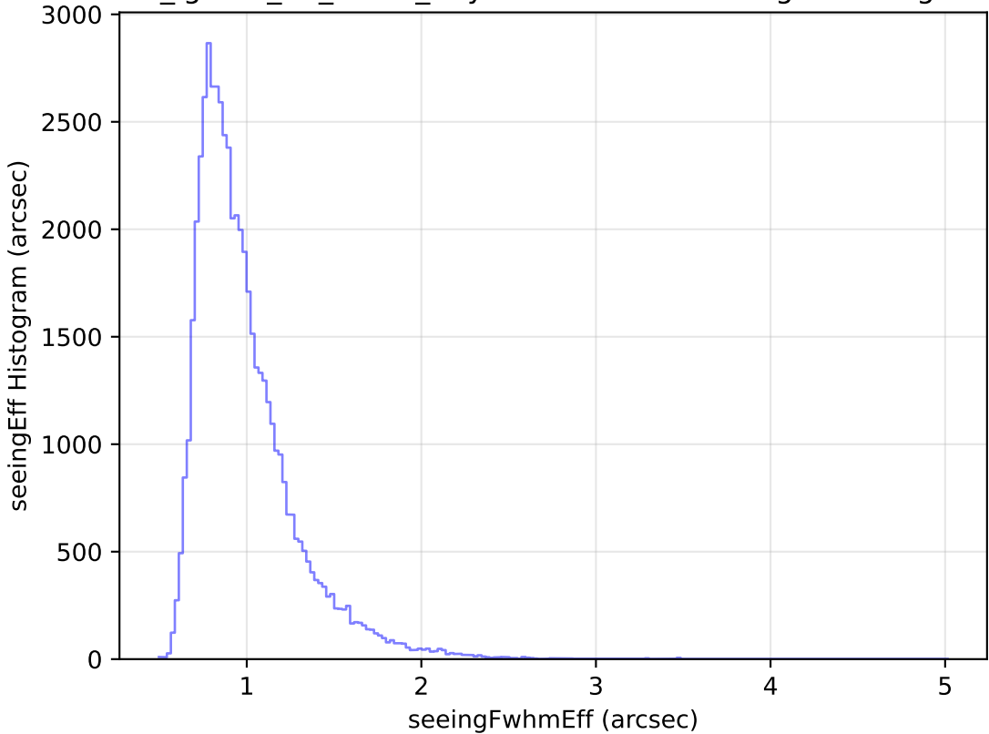
too_ignore_10_1v3.4_10yrs Yr 1 i band: seeingEff Histogram
