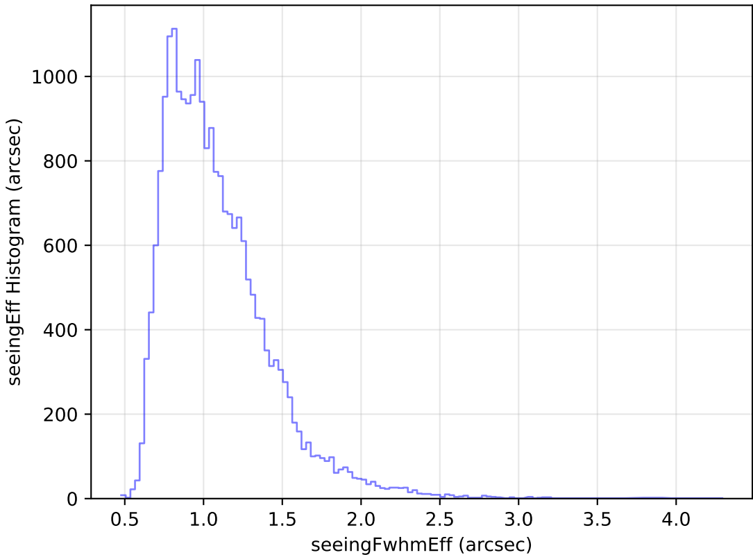
too_ignore_10_1v3.4_10yrs Yr 1 g band: seeingEff Histogram
