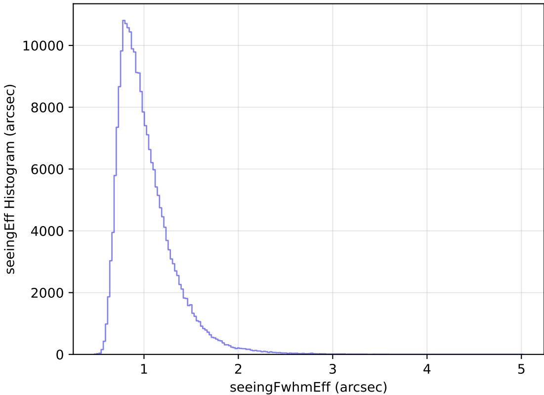
too_ignore_10_1v3.4_10yrs Yr 1 all bands: seeingEff Histogram
