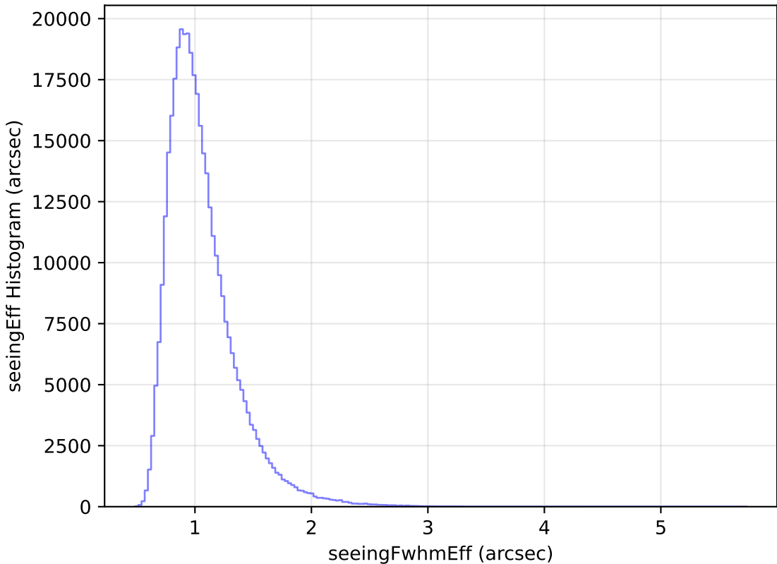
too_ignore_10_1v3.4_10yrs WFD y band: seeingEff Histogram
