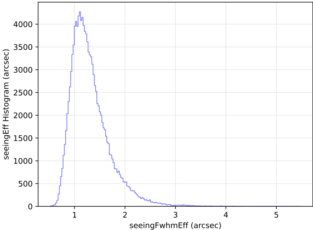
too_ignore_10_1v3.4_10yrs WFD u band: seeingEff Histogram
