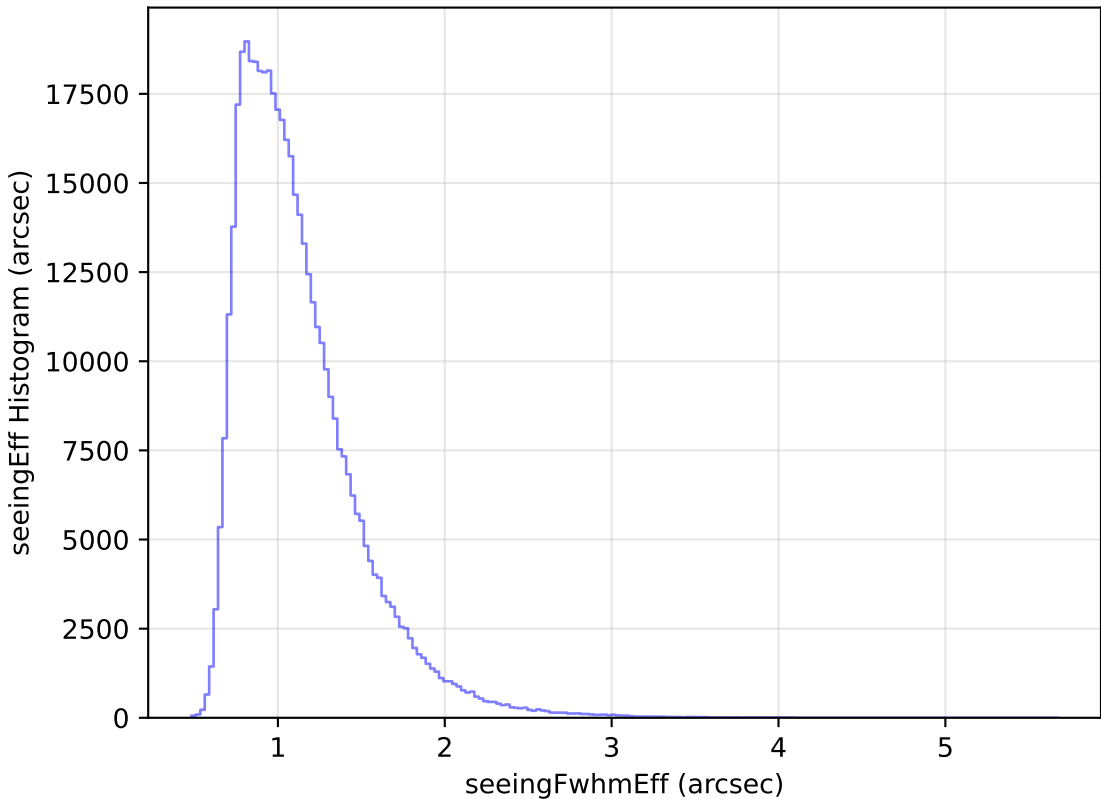
too_ignore_10_1v3.4_10yrs WFD r band: seeingEff Histogram
