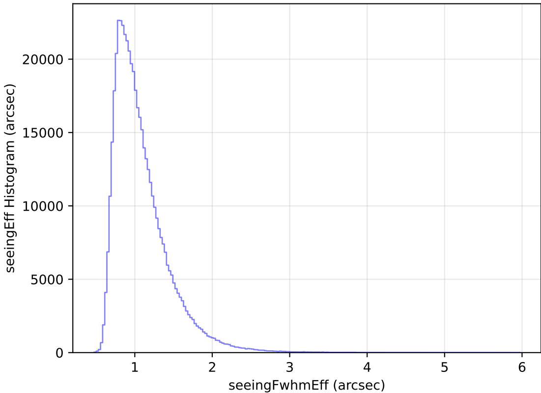
too_ignore_10_1v3.4_10yrs WFD i band: seeingEff Histogram
