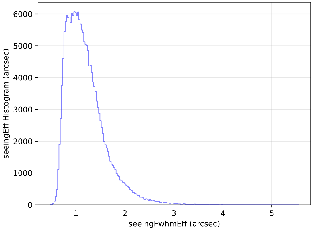
too_ignore_10_1v3.4_10yrs WFD g band: seeingEff Histogram
