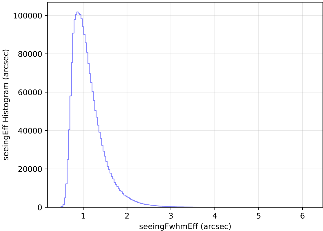
too_ignore_10_1v3.4_10yrs WFD all bands: seeingEff Histogram
