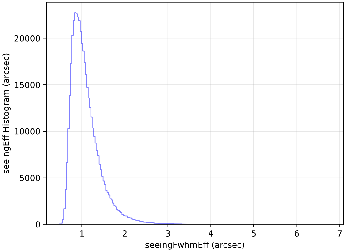
too_ignore_10_1v3.4_10yrs All sky z band: seeingEff Histogram
