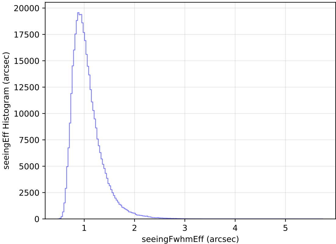
too_ignore_10_1v3.4_10yrs All sky y band: seeingEff Histogram
