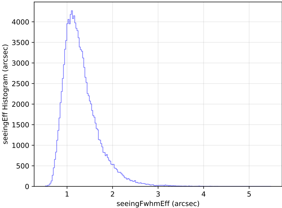
too_ignore_10_1v3.4_10yrs All sky u band: seeingEff Histogram
